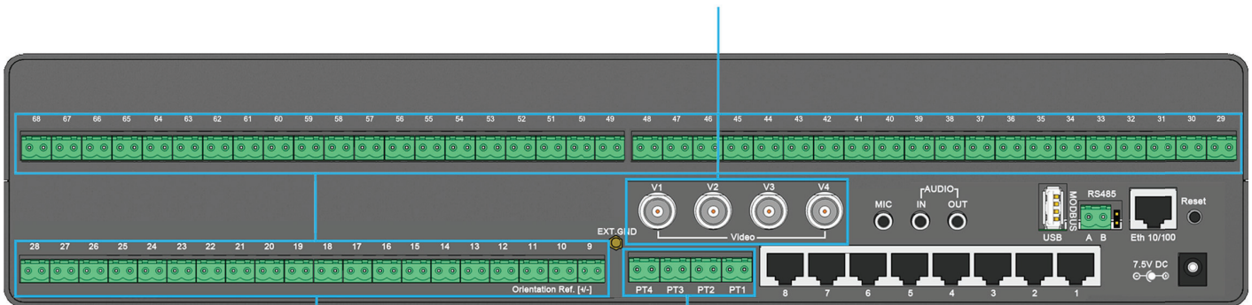
Analog BNC video inputs (5ESVA only). 5ESV comes with USB digital video inputs
